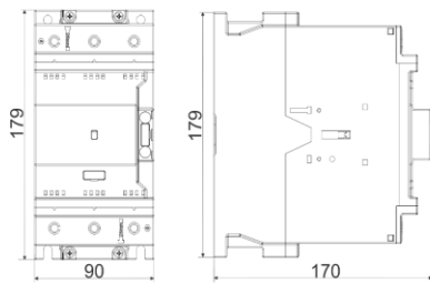
Dimension drawings (mm) CNN 115
