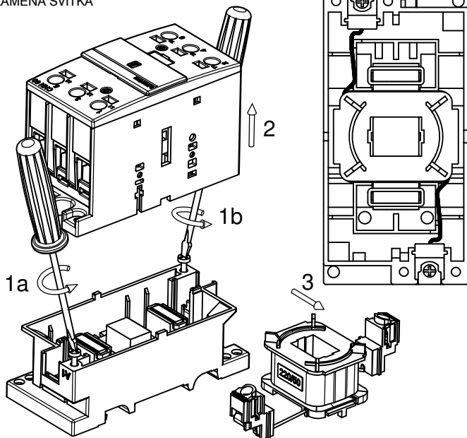
REPLACEMENT OF THE COIL CNN 50, CNN 60, CNN 70, CNN 80, CNN 90 ЗАМЕНА НА КАЛЕМ ZAMENA SVITKA
