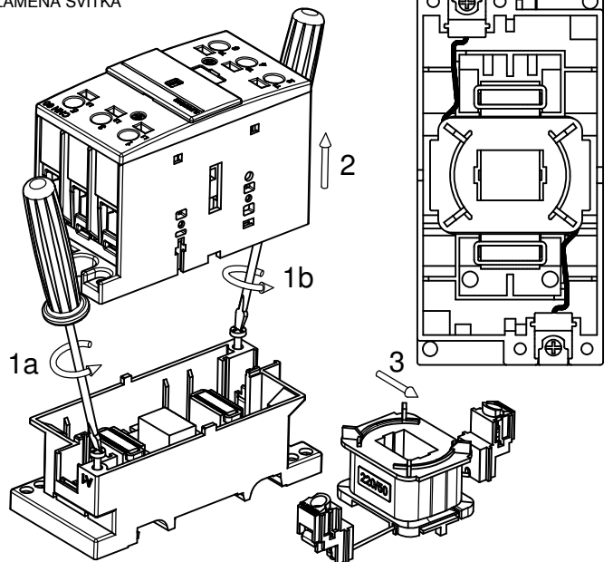
REPLACEMENT OF THE COIL CNN 50, CNN 60, CNN 70, CNN 80, CNN 90 ЗАМЕНА НА КАЛЕМ ZAMENA SVITKA
